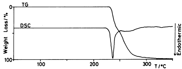
Fig. 7. TG-DSC curves of anti tetrabutylidamide ( 13 ).
